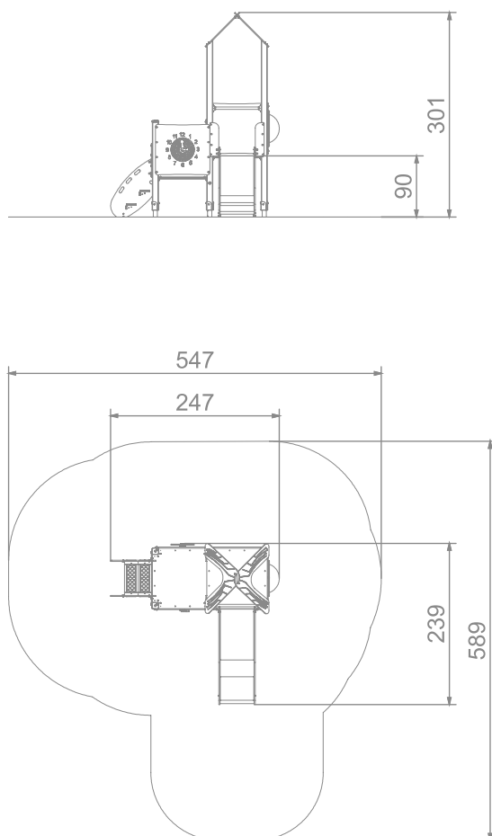
SCALE 1:100
